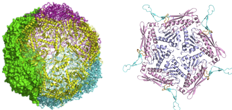
Fig. 2. Crystal structure of EncMh (PDB:6I9G). Left: the 60-meric EncMh with three pentameric units in yellow. Right: a pentamer with protomers in different colors. (For interpretation of the references to color in this figure legend, the reader is referred to the Web version of this article.)
